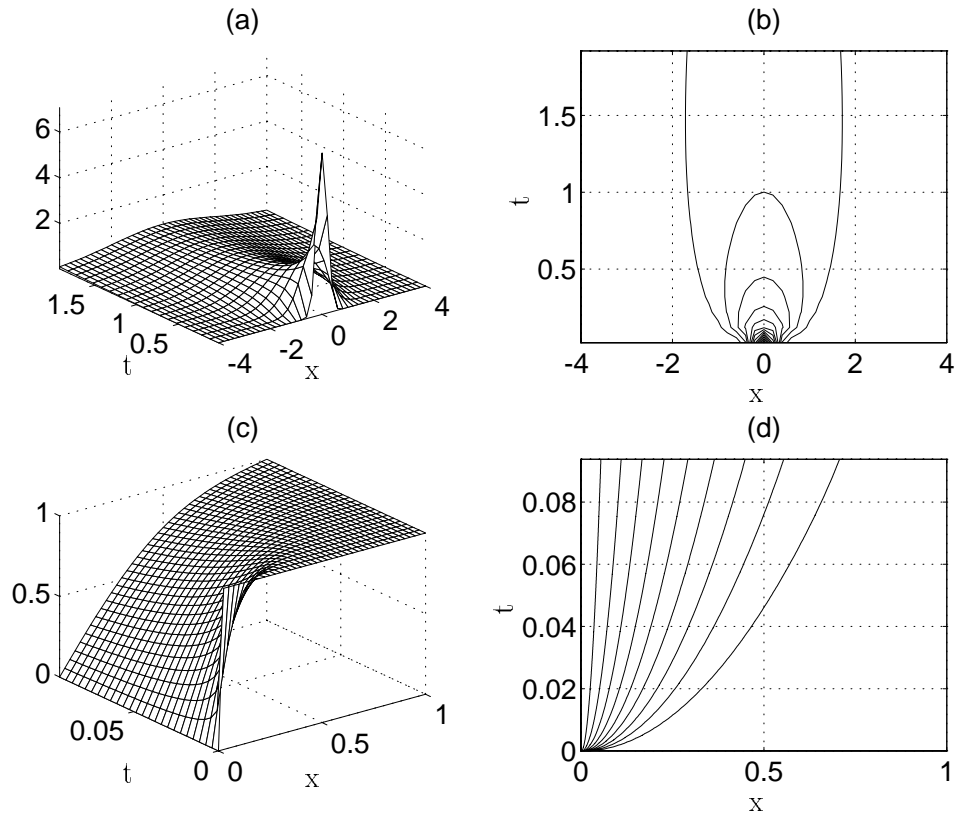
Figure 2: Solutions of the Heat Equation: (a), (b) – the fundamental solution (9) and its contours u = n/2, n = 1, 2, \dots, 14 .
