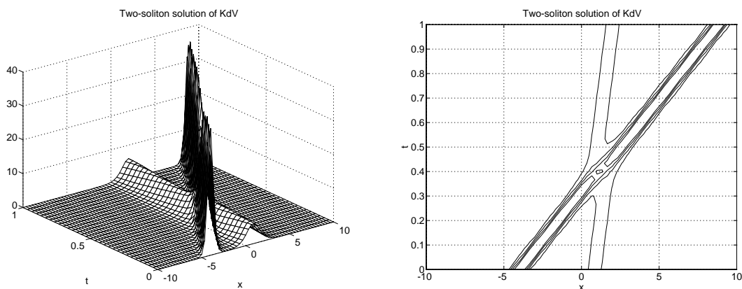
Figure 1: Two-soliton solution of the KdV equation. The right hand figure is a contour plot of that on the left.
